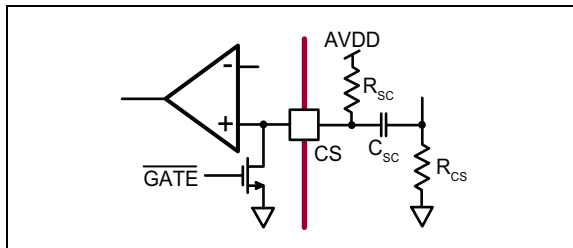
FIGURE 3-1: Slope Compensation.
