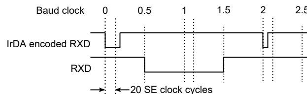
Figure 32-13. IrDA Receive Decoding
