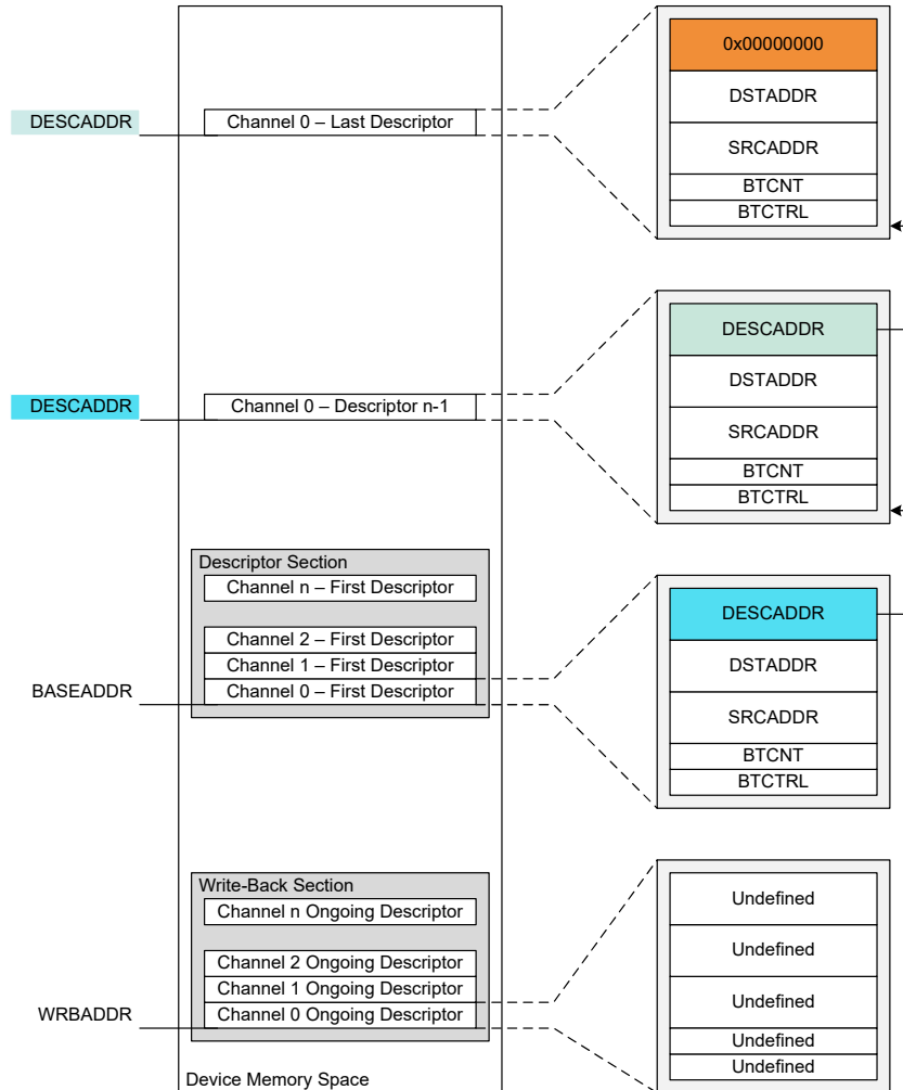
Figure 25-3. Memory Sections
