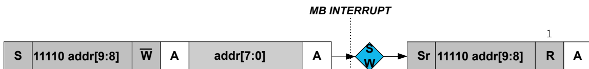
Figure 34-9. 10-bit Address Transmission for a Read Transaction
