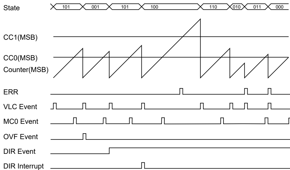
Figure 42-12. Hall Waveforms
