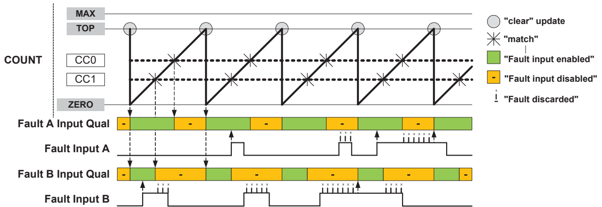
Figure 45-23. Fault Qualification in RAMP1 Operation
