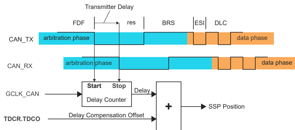
Figure 38-2. Transceiver delay measurement
