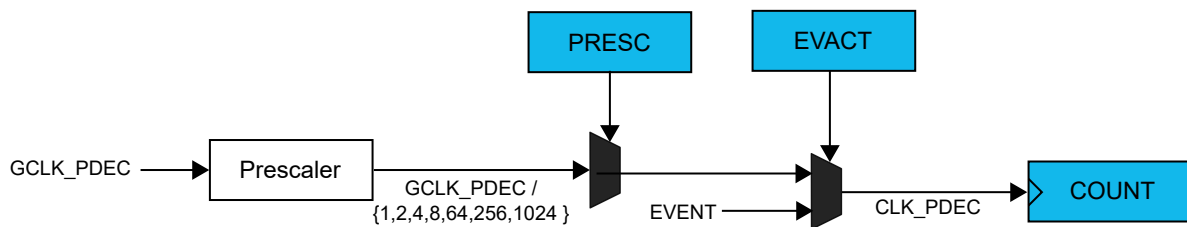
Figure 42-2. Prescaler Selection
