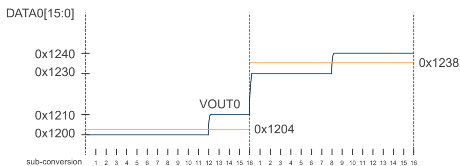
Figure 53-5. DAC Conversions in Dithering Mode
