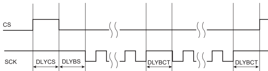
Figure 35-5. Programmable Delay
