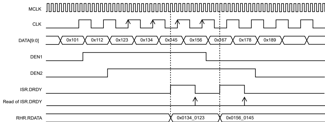
Figure 39-5. PCC Waveforms (ISIZE = 10_BITS, DSIZE = 2_DATA, ALWAYS = 0, HALFS = 0, SCALE = 1)
