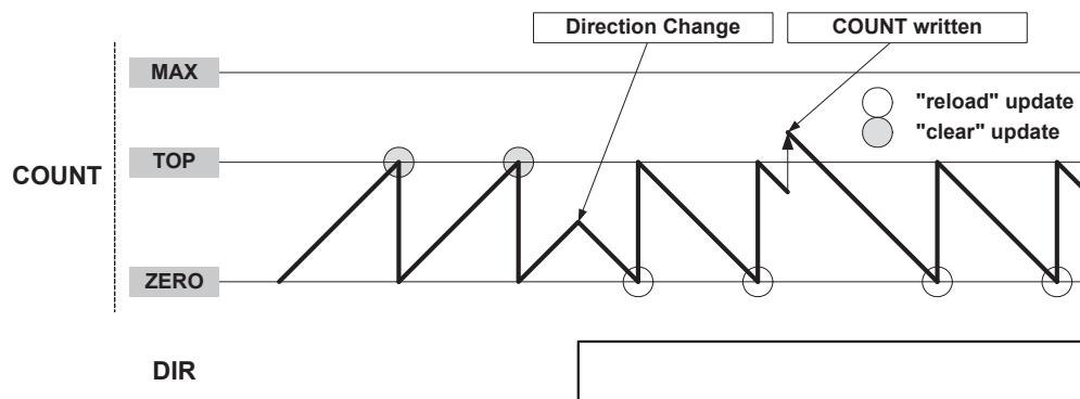
Figure 45-3. Counter Operation
