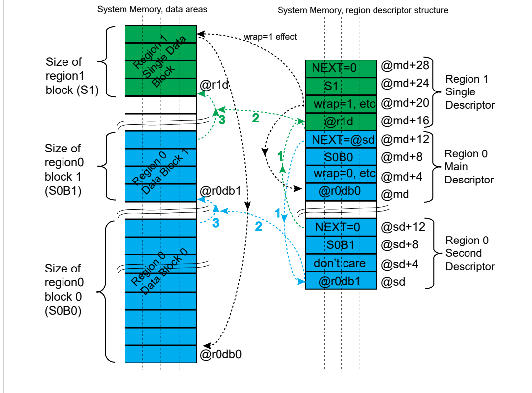
Figure 49-4. Example - Monitoring of 3 Memory Data Blocks (Defined as 2 Regions)
