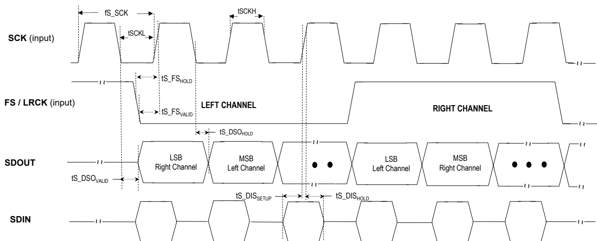
Figure 55-6. I 2 S Client Mode Timing Diagram
