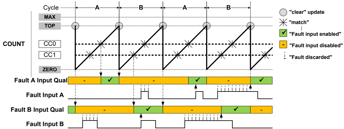
Figure 45-24. Fault Qualification in RAMP2 Operation with Inverted Polarity
