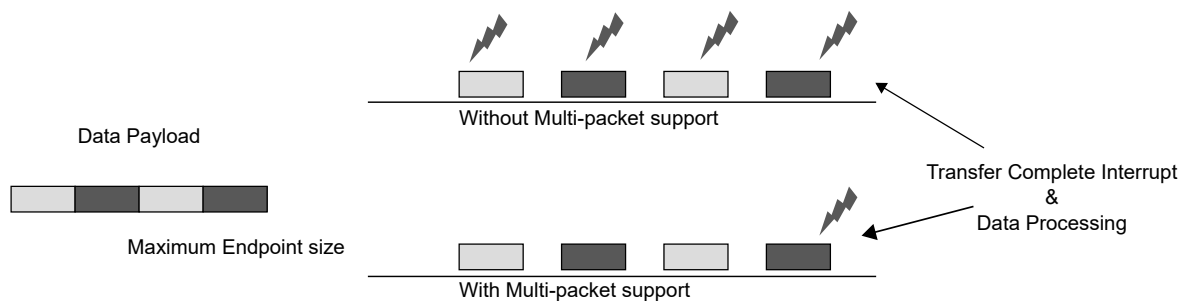
Figure 40-3. Multi-Packet Feature - Reduction of CPU Overhead
