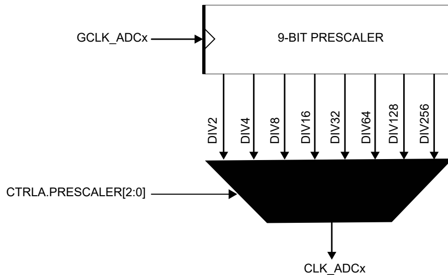
Figure 51-2. ADC Prescaler
