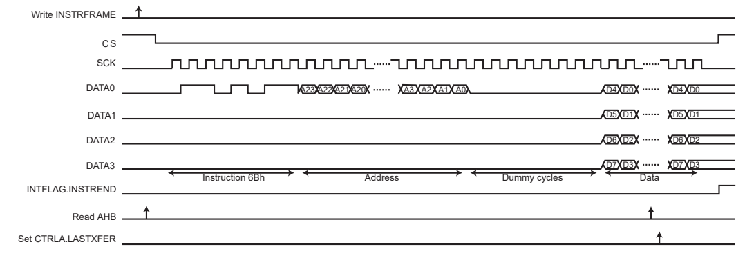
Figure 35-17. Instruction Transmission Waveform 6
