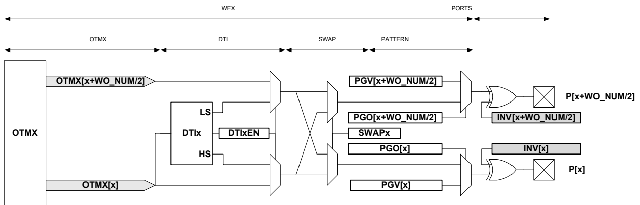
Figure 45-34. Waveform Extension Stage Details
