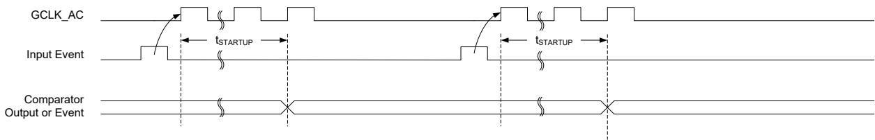
Figure 52-10. Single-Shot SleepWalking
