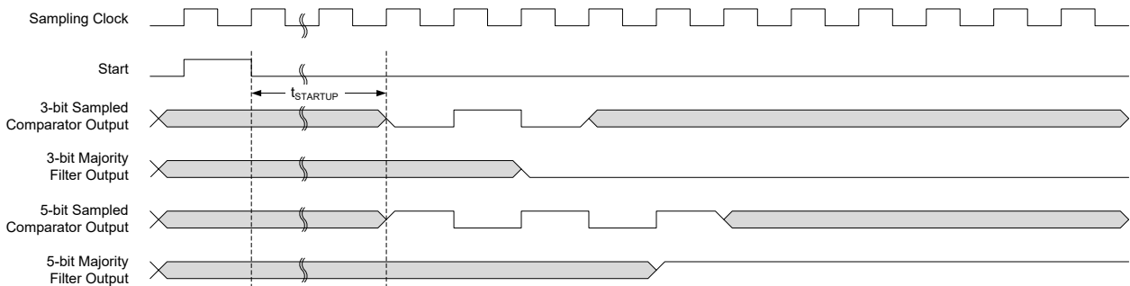
Figure 52-7. Single-Shot Filtering
