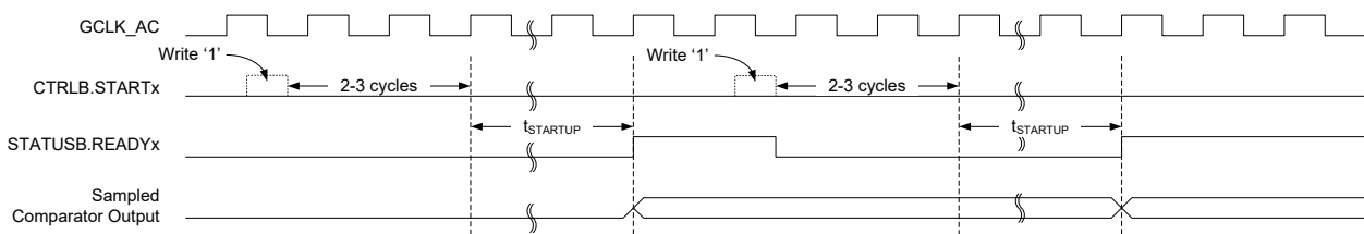
Figure 52-3. Single-Shot Example
