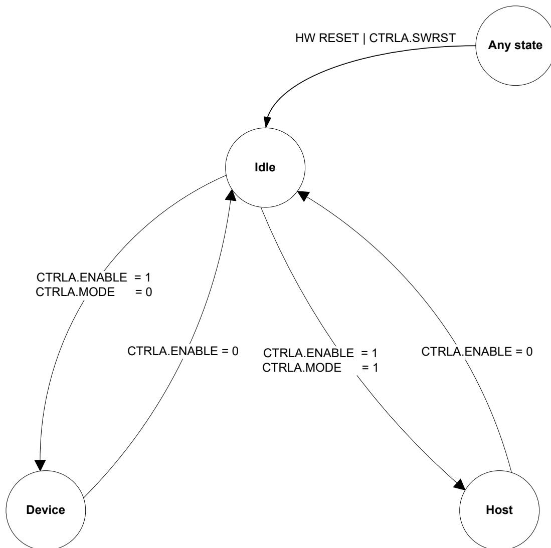
Figure 40-2. General States
