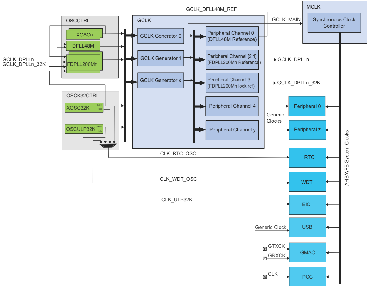
Figure 14-1. Clock Distribution
