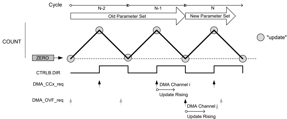
Figure 45-39. DMA Triggers in DSBOOTH Operation Mode and Circular Buffer Enabled
