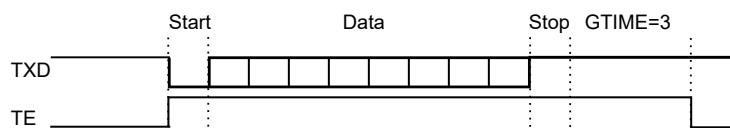
Figure 32-18. Example of TE Drive with Guard Time
