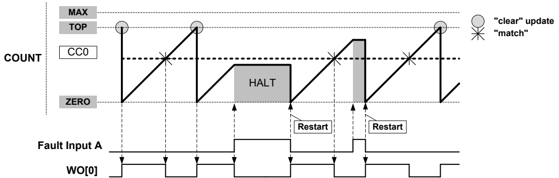
Figure 45-31. Waveform Generation with Fault Qualification, Halt, and Restart Actions
