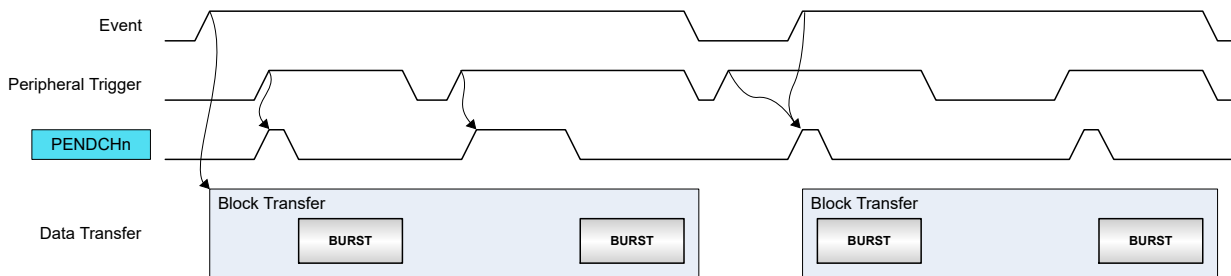
Figure 25-15. Conditional Block Transfer with Burst Peripheral Triggers
