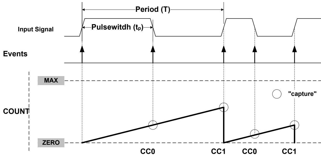
Figure 44-13. PWP Capture
