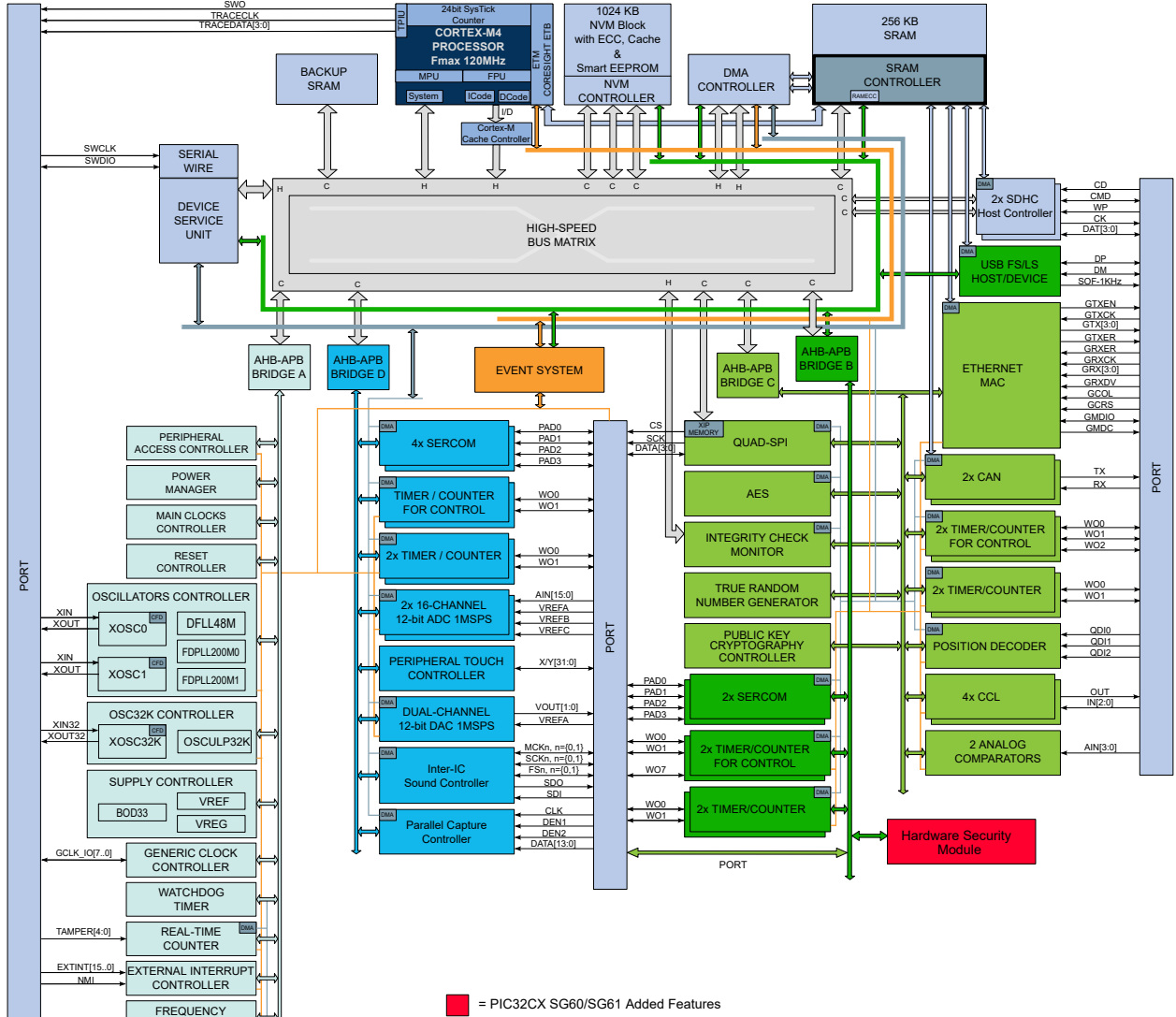
Figure 3-1. PIC32CX SG41/SG60/SG61 Block Diagram
