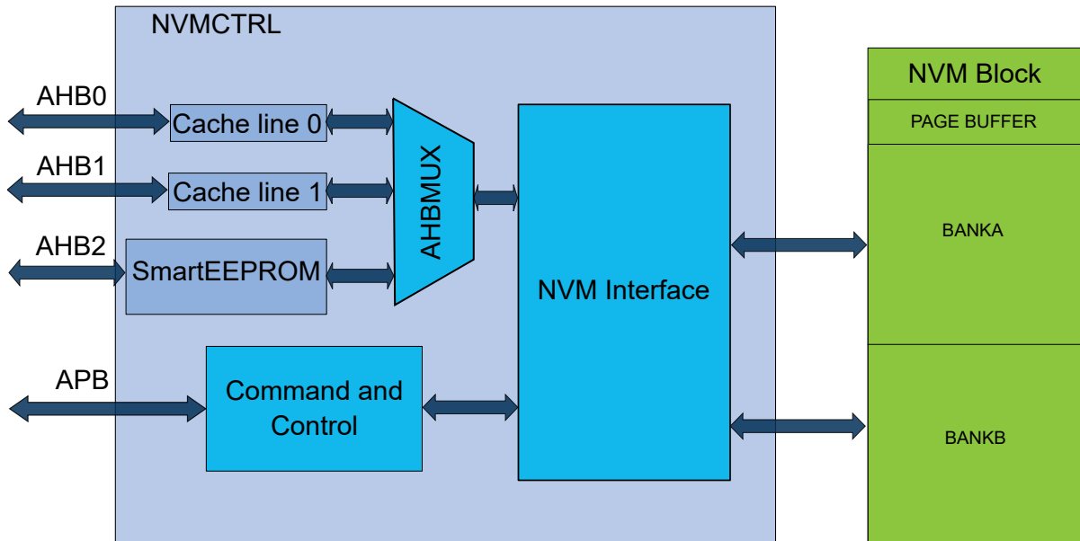
Figure 27-1. Block Diagram
