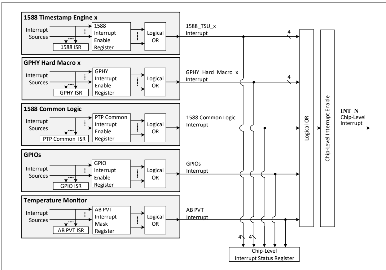
FIGURE 5-14: INTERRUPT STRUCTURE
