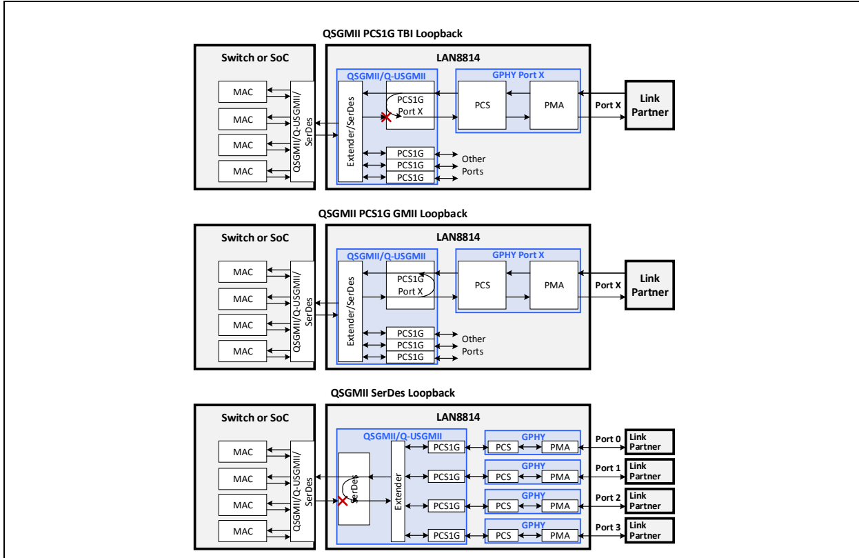
FIGURE 5-12: QSGMII/Q-USGMII LOOPBACK
