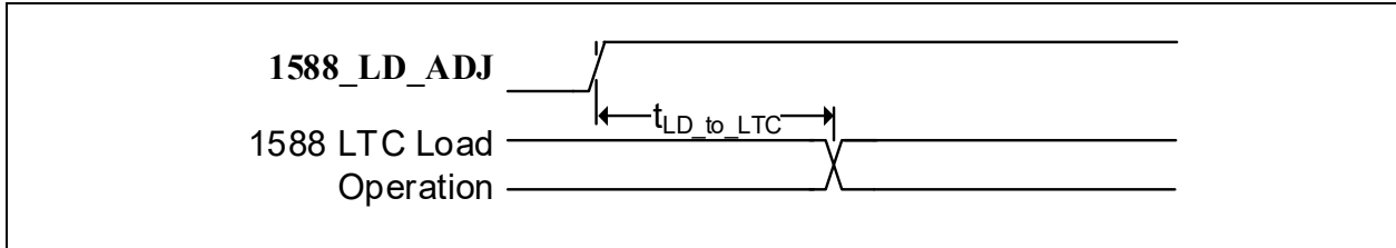
FIGURE 6-10: 1588_LD_ADJ TIMING
