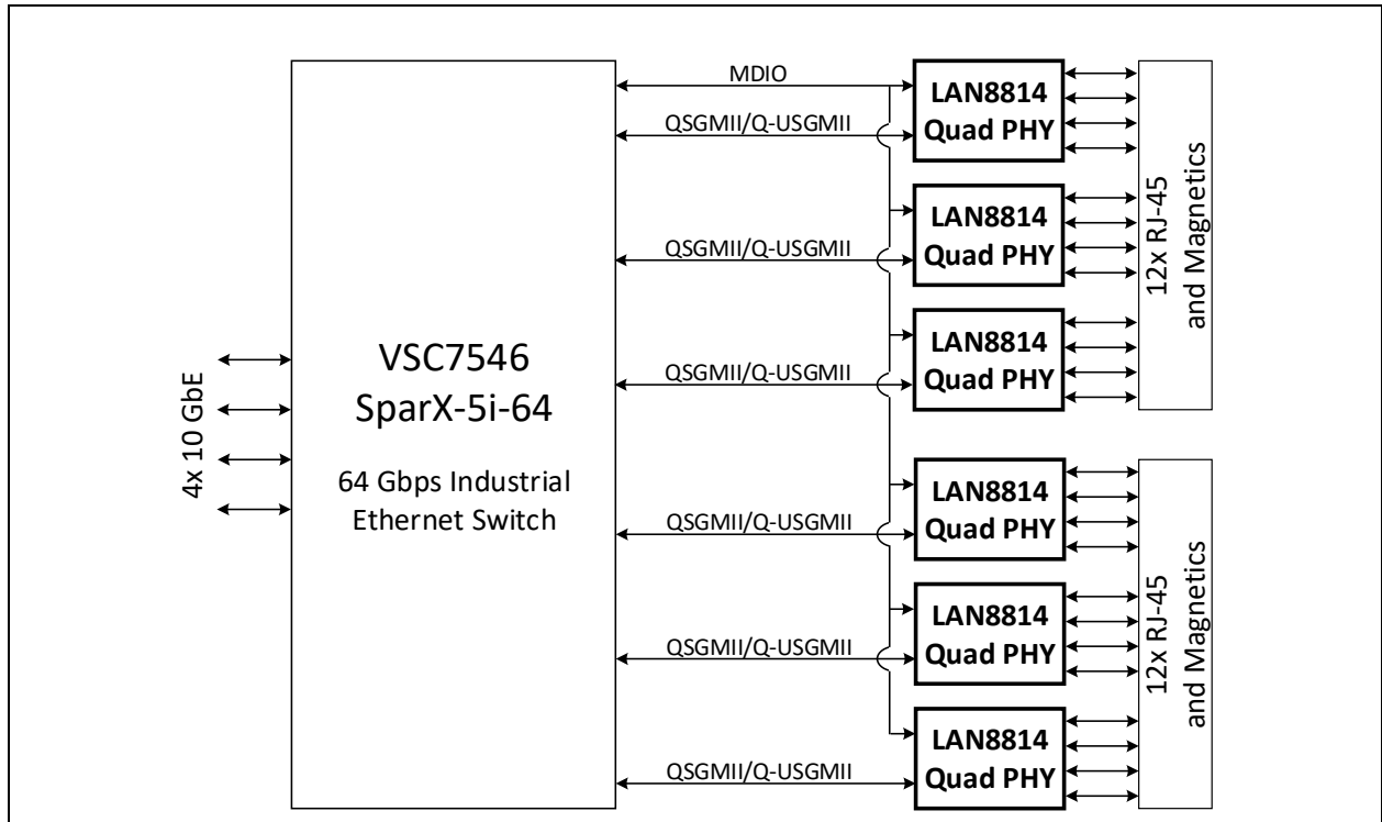
FIGURE 2-2: SWITCH APPLICATION
