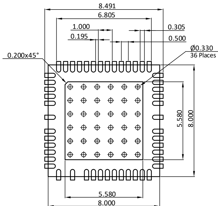
Figure 6-4. Copper Layer (Component Side)
